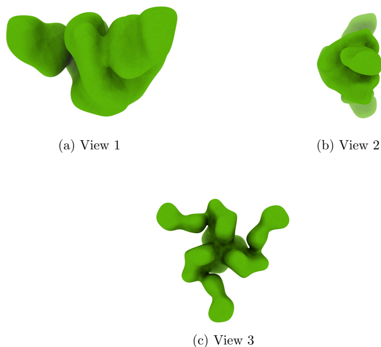
Figure 4: Isosurface at threshold=20.900000. Views generated by ChimeraX at a the following X, Y, Z angles: View 1 (0, -90, -90), View 2 (-90, 0, -90), View 3 (0, 0, 0).
