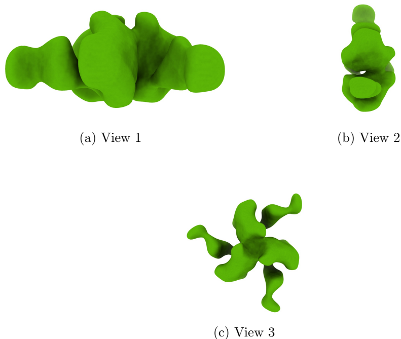
Figure 4: Isosurface at threshold=4.610000. Views generated by ChimeraX at a the following X, Y, Z angles: View 1 (0, -90, -90), View 2 (-90, 0, -90), View 3 (0, 0, 0).
