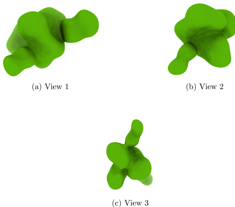
Figure 4: Isosurface at threshold=3.470000. Views generated by ChimeraX at a the following X, Y, Z angles: View 1 (0, -90, -90), View 2 (-90, 0, -90), View 3 (0, 0, 0).
