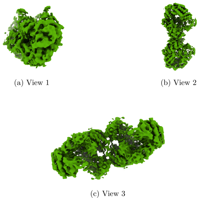
Figure 4: Isosurface at threshold=0.036000. Views generated by ChimeraX at a the following X, Y, Z angles: View 1 (0, -90, -90), View 2 (-90, 0, -90), View 3 (0, 0, 0).
