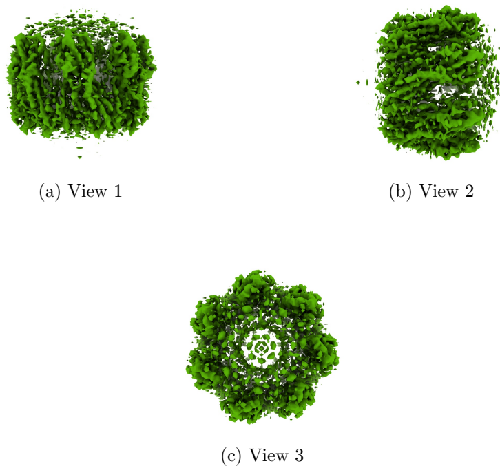
Figure 4: Isosurface at threshold=0.051600. Views generated by ChimeraX at a the following X, Y, Z angles: View 1 (0, -90, -90), View 2 (-90, 0, -90), View 3 (0, 0, 0).
