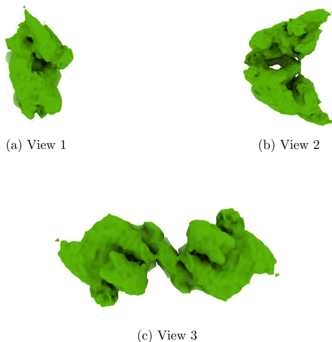
Figure 4: Isosurface at threshold=0.006000. Views generated by ChimeraX at a the following X, Y, Z angles: View 1 (0, -90, -90), View 2 (-90, 0, -90), View 3 (0, 0, 0).
