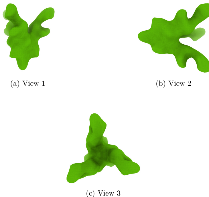
Figure 4: Isosurface at threshold=5.020000. Views generated by ChimeraX at a the following X, Y, Z angles: View 1 (0, -90, -90), View 2 (-90, 0, -90), View 3 (0, 0, 0).
