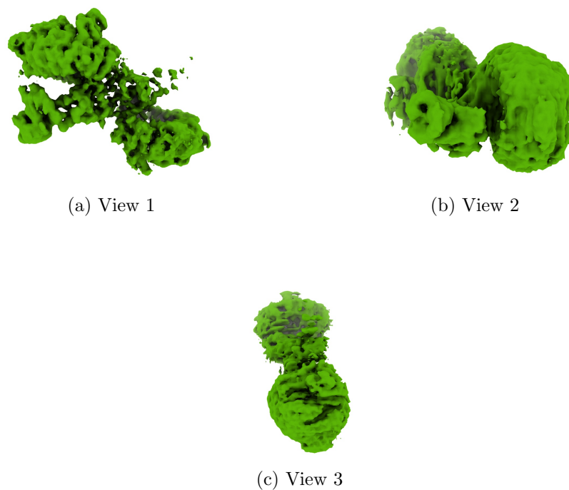
Figure 4: Isosurface at threshold=0.001260. Views generated by ChimeraX at a the following X, Y, Z angles: View 1 (0, -90, -90), View 2 (-90, 0, -90), View 3 (0, 0, 0).
