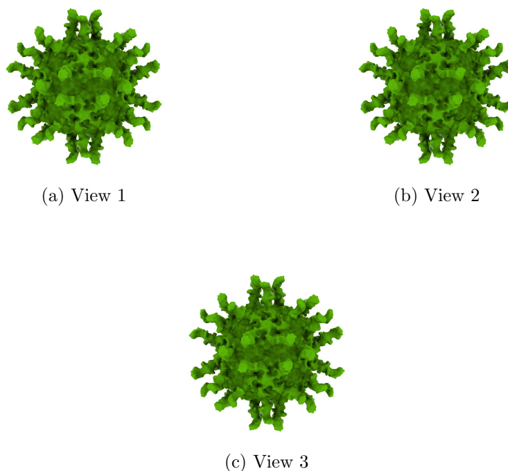
Figure 4: Isosurface at threshold=53.000000. Views generated by ChimeraX at a the following X, Y, Z angles: View 1 (0, -90, -90), View 2 (-90, 0, -90), View 3 (0, 0, 0).
