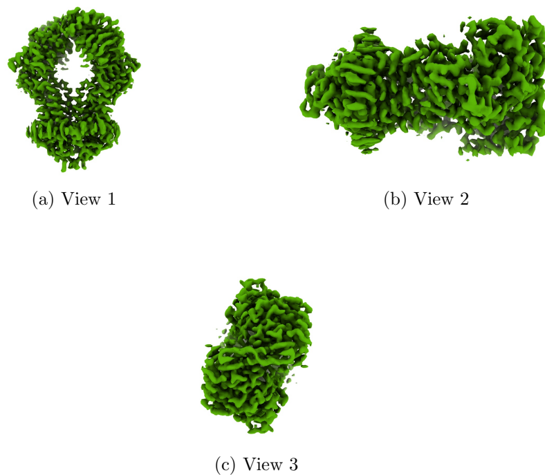
Figure 4: Isosurface at threshold=0.054200. Views generated by ChimeraX at a the following X, Y, Z angles: View 1 (0, -90, -90), View 2 (-90, 0, -90), View 3 (0, 0, 0).
