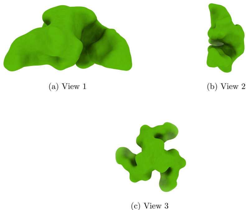
Figure 4: Isosurface at threshold=18.000000. Views generated by ChimeraX at a the following X, Y, Z angles: View 1 (0, -90, -90), View 2 (-90, 0, -90), View 3 (0, 0, 0).
