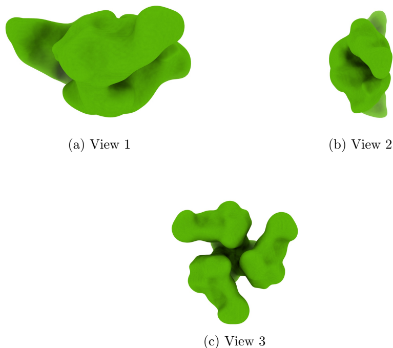
Figure 4: Isosurface at threshold=14.000000. Views generated by ChimeraX at a the following X, Y, Z angles: View 1 (0, -90, -90), View 2 (-90, 0, -90), View 3 (0, 0, 0).
