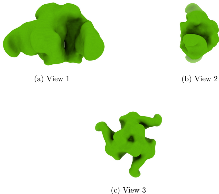
Figure 4: Isosurface at threshold=3.470000. Views generated by ChimeraX at a the following X, Y, Z angles: View 1 (0, -90, -90), View 2 (-90, 0, -90), View 3 (0, 0, 0).
