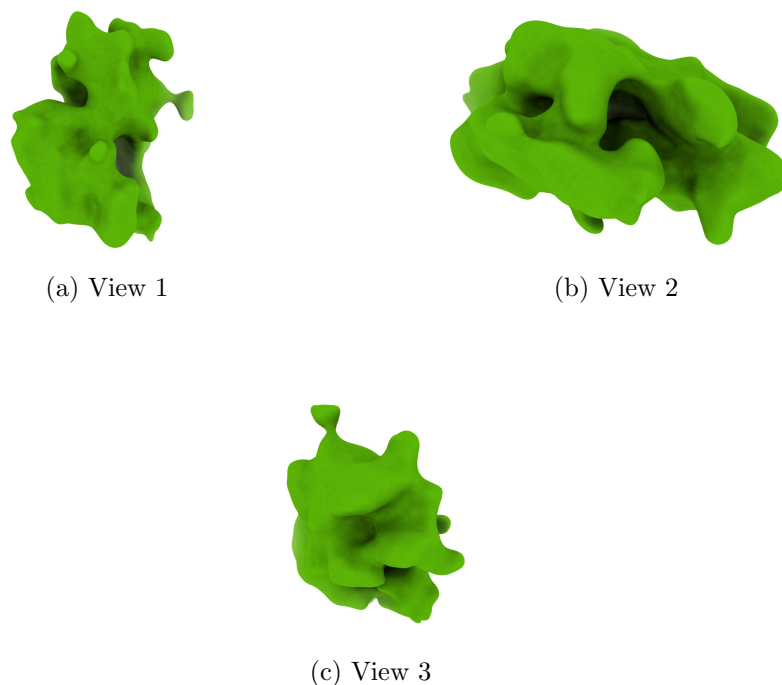
Figure 4: Isosurface at threshold=3.900000. Views generated by ChimeraX at a the following X, Y, Z angles: View 1 (0, -90, -90), View 2 (-90, 0, -90), View 3 (0, 0, 0).
