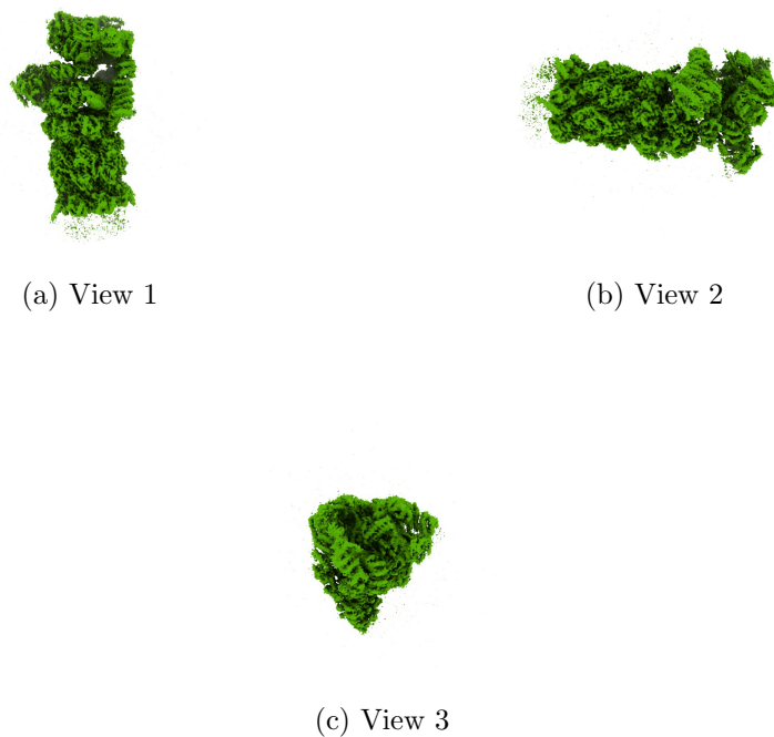
Figure 4: Isosurface at threshold=0.093900. Views generated by ChimeraX at a the following X, Y, Z angles: View 1 (0, -90, -90), View 2 (-90, 0, -90), View 3 (0, 0, 0).
