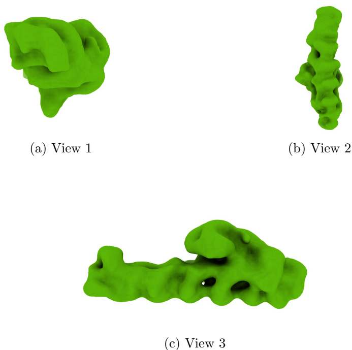
Figure 4: Isosurface at threshold=2.140000. Views generated by ChimeraX at a the following X, Y, Z angles: View 1 (0, -90, -90), View 2 (-90, 0, -90), View 3 (0, 0, 0).
