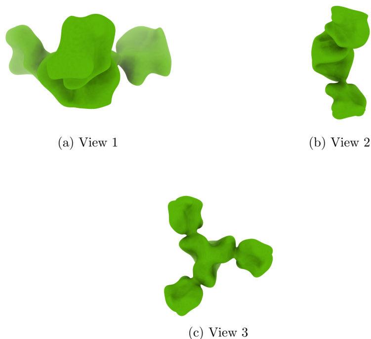
Figure 4: Isosurface at threshold=14.100000. Views generated by ChimeraX at a the following X, Y, Z angles: View 1 (0, -90, -90), View 2 (-90, 0, -90), View 3 (0, 0, 0).
