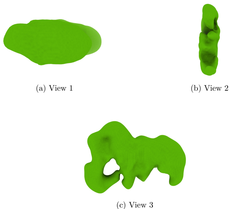
Figure 4: Isosurface at threshold=0.239000. Views generated by ChimeraX at a the following X, Y, Z angles: View 1 (0, -90, -90), View 2 (-90, 0, -90), View 3 (0, 0, 0).
