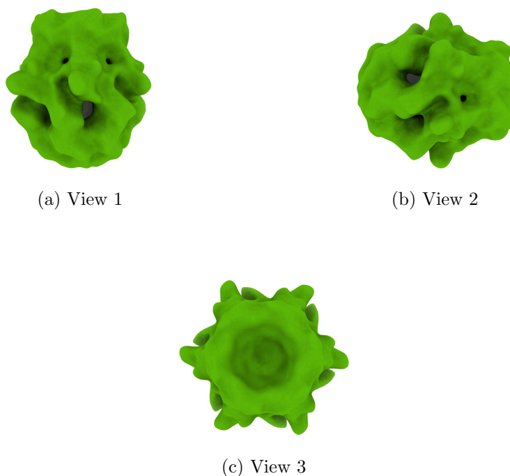
Figure 4: Isosurface at threshold=1.450000. Views generated by ChimeraX at a the following X, Y, Z angles: View 1 (0, -90, -90), View 2 (-90, 0, -90), View 3 (0, 0, 0).
