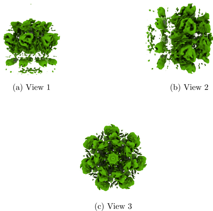
Figure 4: Isosurface at threshold=0.031800. Views generated by ChimeraX at a the following X, Y, Z angles: View 1 (0, -90, -90), View 2 (-90, 0, -90), View 3 (0, 0, 0).
