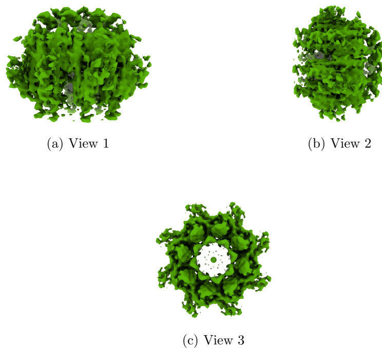
Figure 4: Isosurface at threshold=0.098600. Views generated by ChimeraX at a the following X, Y, Z angles: View 1 (0, -90, -90), View 2 (-90, 0, -90), View 3 (0, 0, 0).
