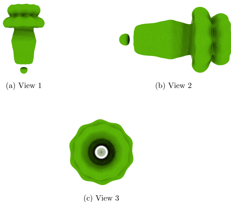
Figure 4: Isosurface at threshold=0.028000. Views generated by ChimeraX at the following X, Y, Z angles: View 1 (0, -90, -90), View 2 (-90, 0, -90), View 3 (0, 0, 0).
