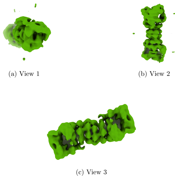
Figure 4: Isosurface at threshold=3.900000. Views generated by ChimeraX at a the following X, Y, Z angles: View 1 (0, -90, -90), View 2 (-90, 0, -90), View 3 (0, 0, 0).
