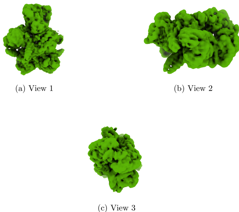
Figure 4: Isosurface at threshold=0.088700. Views generated by ChimeraX at a the following X, Y, Z angles: View 1 (0, -90, -90), View 2 (-90, 0, -90), View 3 (0, 0, 0).
