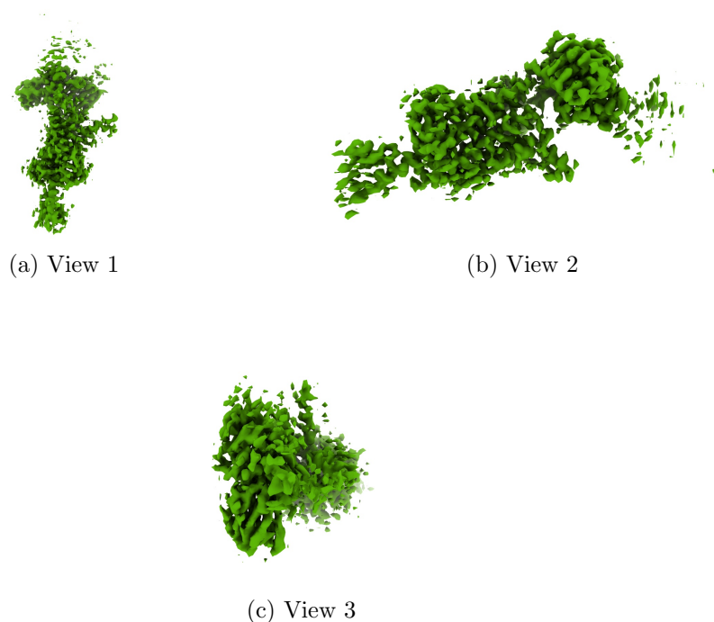
Figure 4: Isosurface at threshold=0.338000. Views generated by ChimeraX at a the following X, Y, Z angles: View 1 (0, -90, -90), View 2 (-90, 0, -90), View 3 (0, 0, 0).
