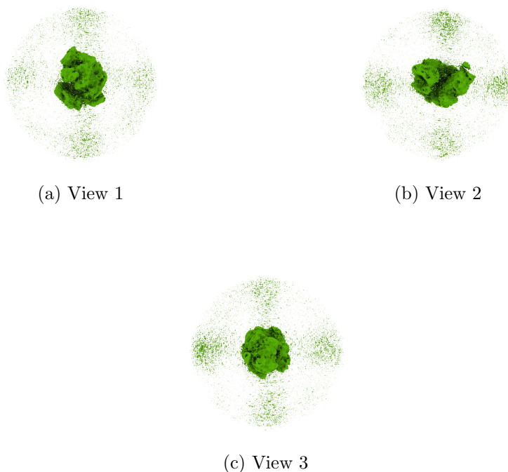
Figure 4: Isosurface at threshold=0.067500. Views generated by ChimeraX at a the following X, Y, Z angles: View 1 (0, -90, -90), View 2 (-90, 0, -90), View 3 (0, 0, 0).
