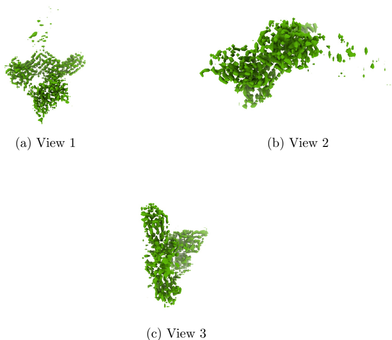
Figure 4: Isosurface at threshold=0.279000. Views generated by ChimeraX at a the following X, Y, Z angles: View 1 (0, -90, -90), View 2 (-90, 0, -90), View 3 (0, 0, 0).
