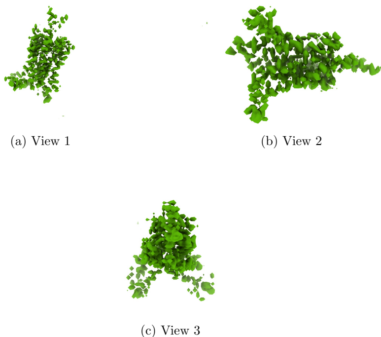
Figure 4: Isosurface at threshold=0.246000. Views generated by ChimeraX at a the following X, Y, Z angles: View 1 (0, -90, -90), View 2 (-90, 0, -90), View 3 (0, 0, 0).
