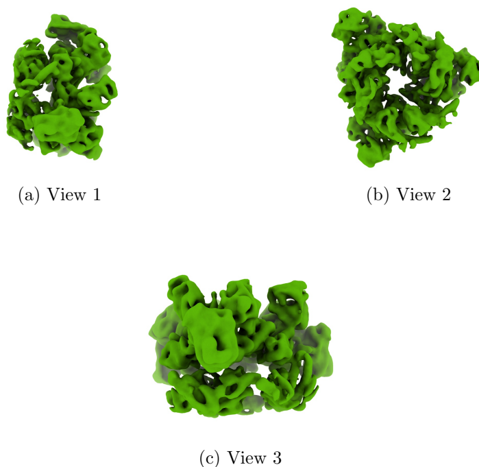
Figure 4: Isosurface at threshold=0.012300. Views generated by ChimeraX at the following X, Y, Z angles: View 1 (0, -90, -90), View 2 (-90, 0, -90), View 3 (0, 0, 0).
