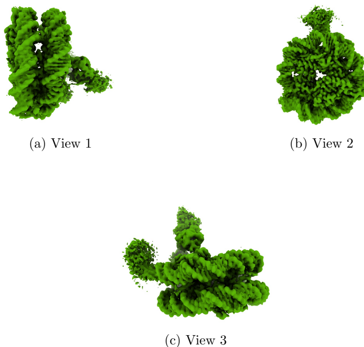
Figure 4: Isosurface at threshold=0.001390. Views generated by ChimeraX at a the following X, Y, Z angles: View 1 (0, -90, -90), View 2 (-90, 0, -90), View 3 (0, 0, 0).
