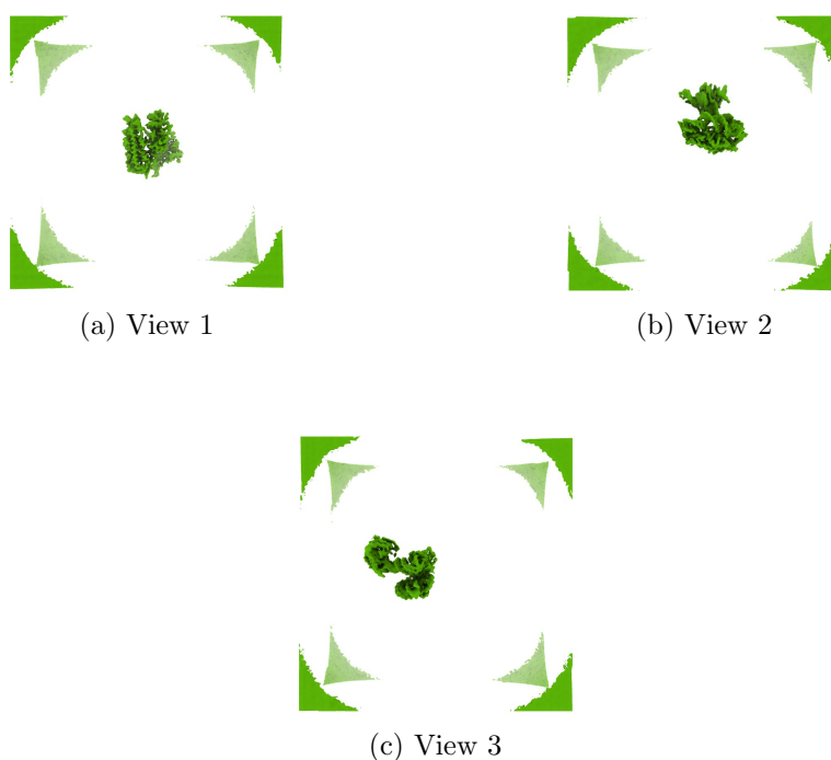
Figure 4: Isosurface at threshold=0.002270. Views generated by ChimeraX at a the following X, Y, Z angles: View 1 (0, -90, -90), View 2 (-90, 0, -90), View 3 (0, 0, 0).
