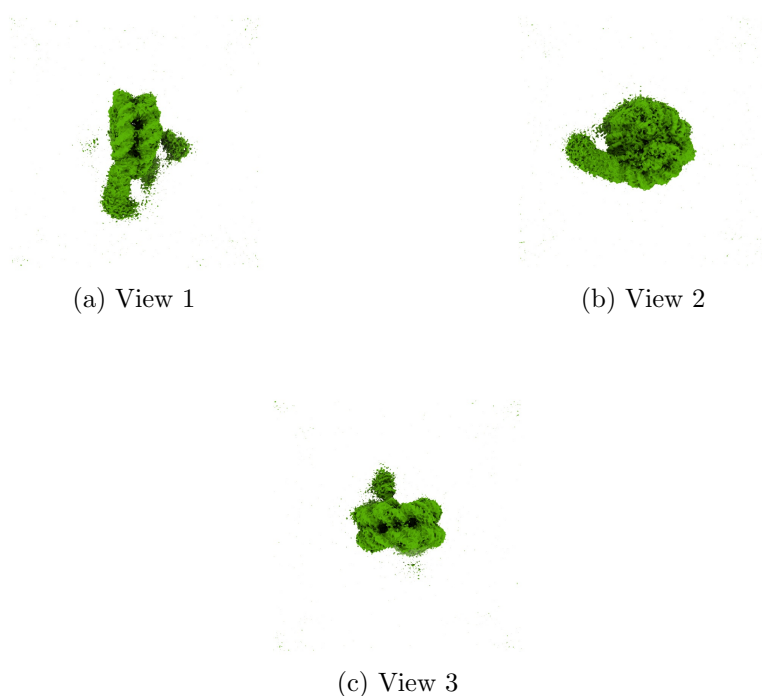
Figure 4: Isosurface at threshold=0.000400. Views generated by ChimeraX at a the following X, Y, Z angles: View 1 (0, -90, -90), View 2 (-90, 0, -90), View 3 (0, 0, 0).
