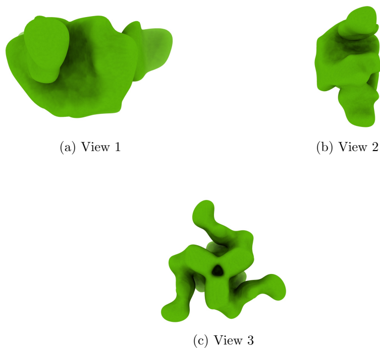
Figure 4: Isosurface at threshold=12.300000. Views generated by ChimeraX at a the following X, Y, Z angles: View 1 (0, -90, -90), View 2 (-90, 0, -90), View 3 (0, 0, 0).
