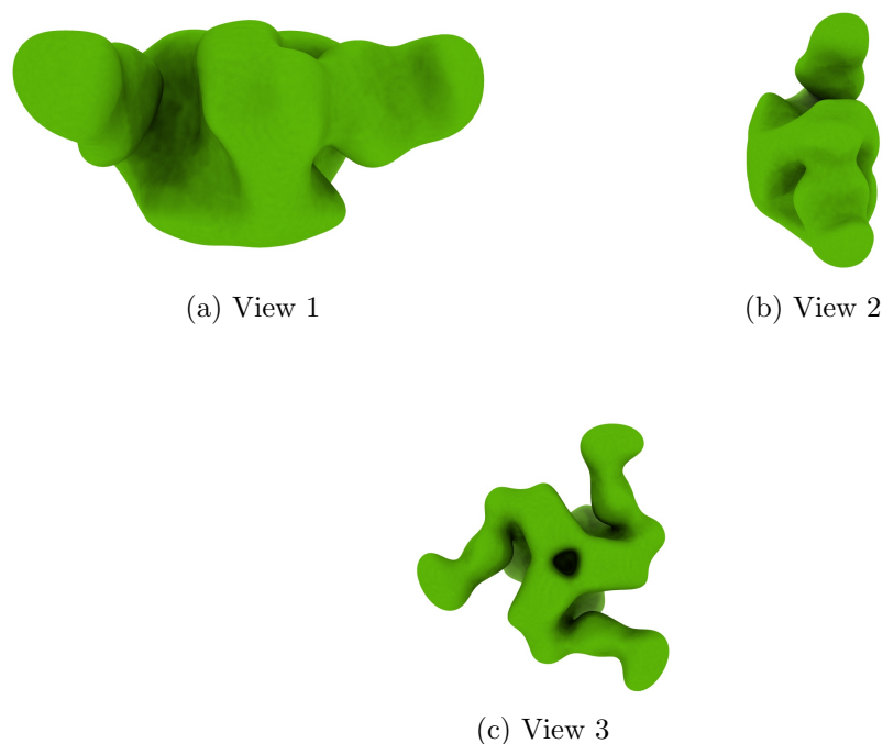
Figure 4: Isosurface at threshold=20.000000. Views generated by ChimeraX at a the following X, Y, Z angles: View 1 (0, -90, -90), View 2 (-90, 0, -90), View 3 (0, 0, 0).
