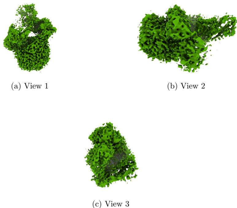
Figure 4: Isosurface at threshold=0.050300. Views generated by ChimeraX at a the following X, Y, Z angles: View 1 (0, -90, -90), View 2 (-90, 0, -90), View 3 (0, 0, 0).
