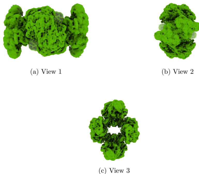
Figure 4: Isosurface at threshold=0.014300. Views generated by ChimeraX at a the following X, Y, Z angles: View 1 (0, -90, -90), View 2 (-90, 0, -90), View 3 (0, 0, 0).
