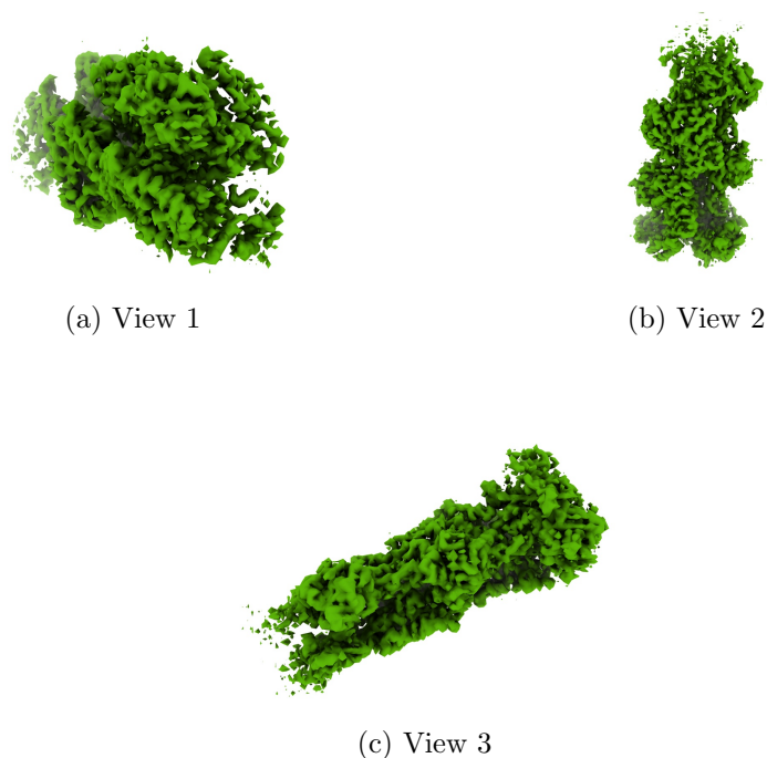
Figure 4: Isosurface at threshold=0.188000. Views generated by ChimeraX at a the following X, Y, Z angles: View 1 (0, -90, -90), View 2 (-90, 0, -90), View 3 (0, 0, 0).
