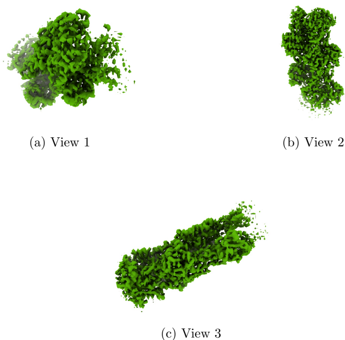
Figure 4: Isosurface at threshold=0.262000. Views generated by ChimeraX at a the following X, Y, Z angles: View 1 (0, -90, -90), View 2 (-90, 0, -90), View 3 (0, 0, 0).
