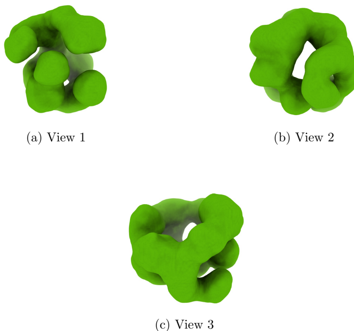
Figure 4: Isosurface at threshold=0.004900. Views generated by ChimeraX at a the following X, Y, Z angles: View 1 (0, -90, -90), View 2 (-90, 0, -90), View 3 (0, 0, 0).
