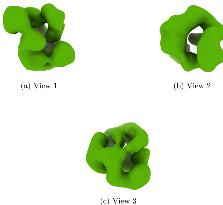
Figure 4: Isosurface at threshold=0.007900. Views generated by ChimeraX at a the following X, Y, Z angles: View 1 (0, -90, -90), View 2 (-90, 0, -90), View 3 (0, 0, 0).
