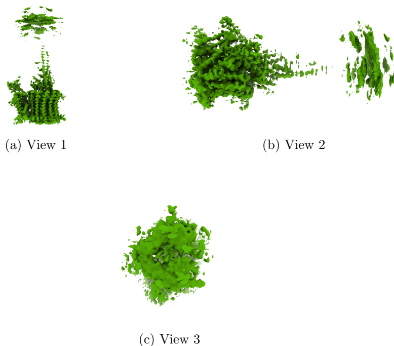
Figure 4: Isosurface at threshold=0.008300. Views generated by ChimeraX at a the following X, Y, Z angles: View 1 (0, -90, -90), View 2 (-90, 0, -90), View 3 (0, 0, 0).
