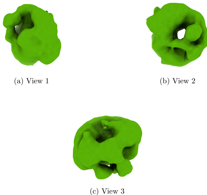
Figure 4: Isosurface at threshold=0.006700. Views generated by ChimeraX at a the following X, Y, Z angles: View 1 (0, -90, -90), View 2 (-90, 0, -90), View 3 (0, 0, 0).
