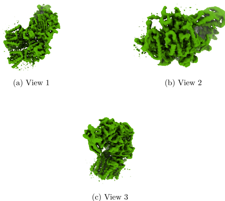
Figure 4: Isosurface at threshold=0.008360. Views generated by ChimeraX at a the following X, Y, Z angles: View 1 (0, -90, -90), View 2 (-90, 0, -90), View 3 (0, 0, 0).
