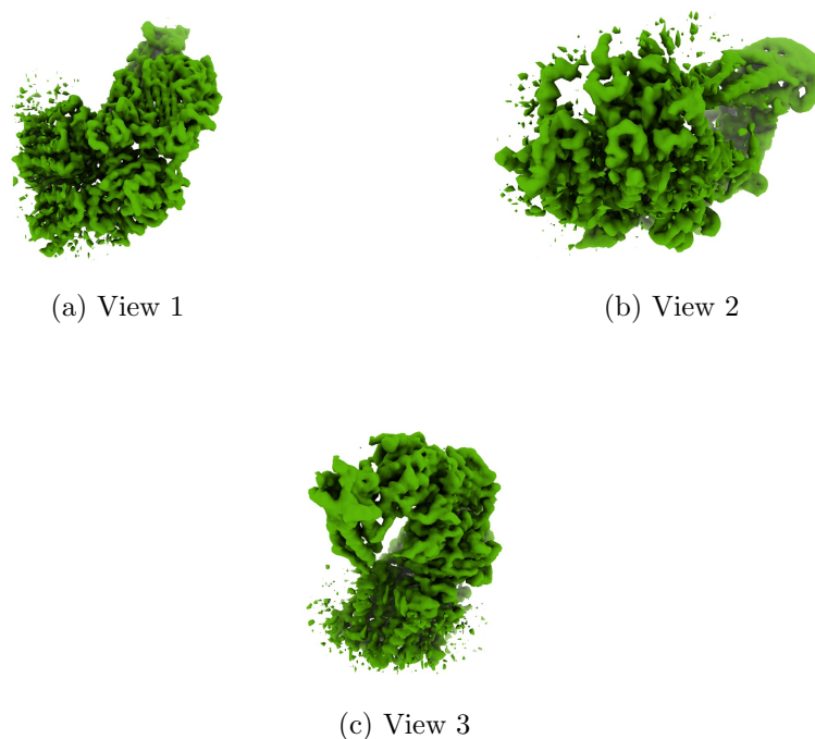
Figure 4: Isosurface at threshold=0.008010. Views generated by ChimeraX at a the following X, Y, Z angles: View 1 (0, -90, -90), View 2 (-90, 0, -90), View 3 (0, 0, 0).
