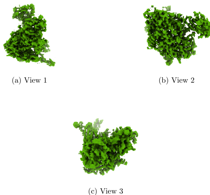
Figure 4: Isosurface at threshold=0.579000. Views generated by ChimeraX at a the following X, Y, Z angles: View 1 (0, -90, -90), View 2 (-90, 0, -90), View 3 (0, 0, 0).
