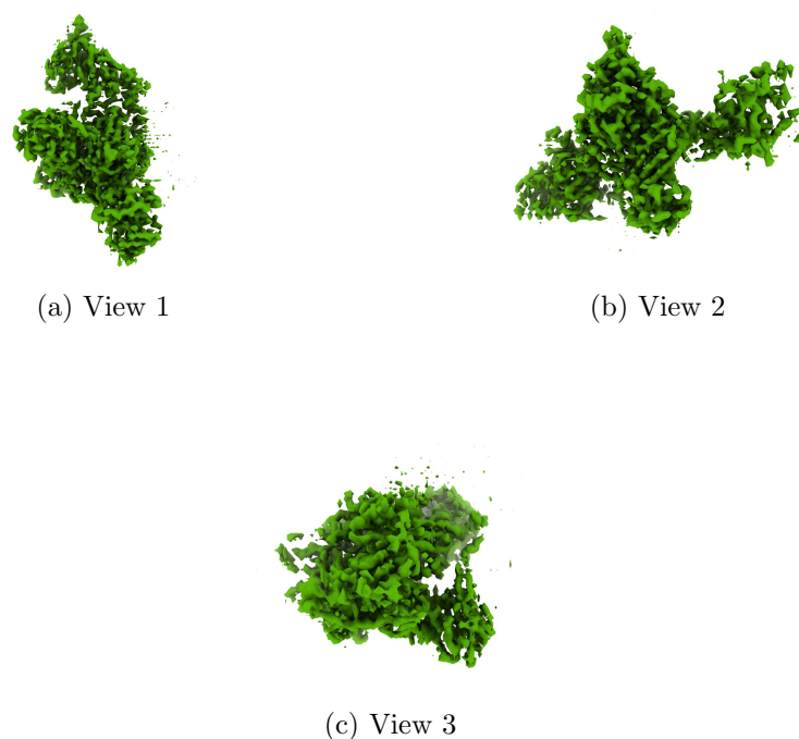
Figure 4: Isosurface at threshold=0.610000. Views generated by ChimeraX at a the following X, Y, Z angles: View 1 (0, -90, -90), View 2 (-90, 0, -90), View 3 (0, 0, 0).
