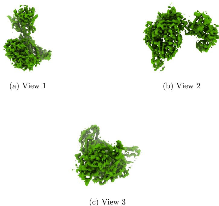
Figure 4: Isosurface at threshold=0.645000. Views generated by ChimeraX at a the following X, Y, Z angles: View 1 (0, -90, -90), View 2 (-90, 0, -90), View 3 (0, 0, 0).
