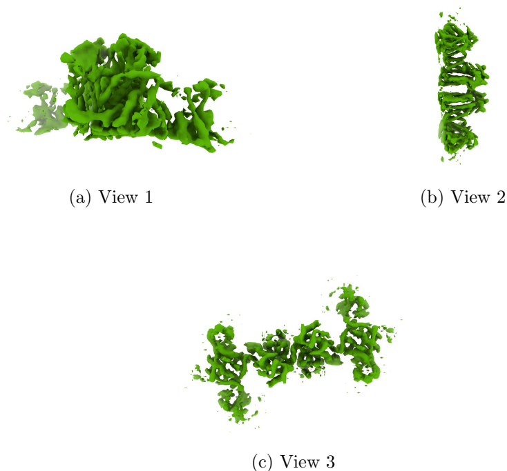
Figure 4: Isosurface at threshold=0.330000. Views generated by ChimeraX at a the following X, Y, Z angles: View 1 (0, -90, -90), View 2 (-90, 0, -90), View 3 (0, 0, 0).
