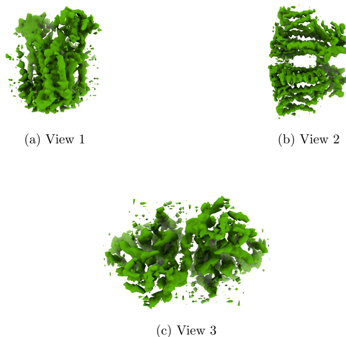
Figure 4: Isosurface at threshold=0.359000. Views generated by ChimeraX at a the following X, Y, Z angles: View 1 (0, -90, -90), View 2 (-90, 0, -90), View 3 (0, 0, 0).
