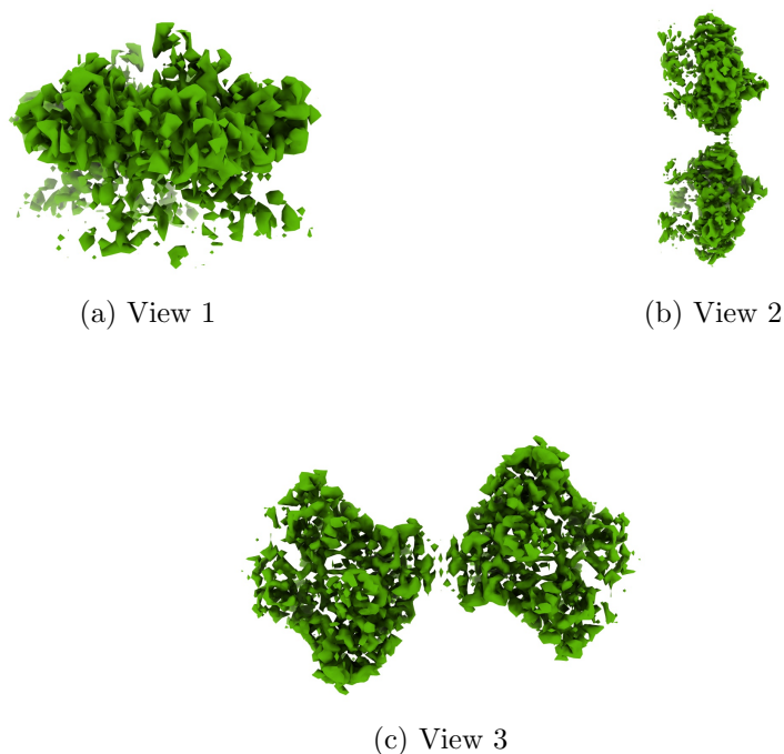
Figure 4: Isosurface at threshold=0.418000. Views generated by ChimeraX at a the following X, Y, Z angles: View 1 (0, -90, -90), View 2 (-90, 0, -90), View 3 (0, 0, 0).
